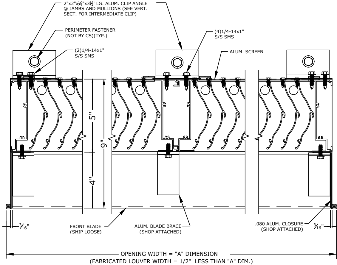
PLAN VIEW (SEE SHEET 2 FOR VERTICAL SECTION) NTS
