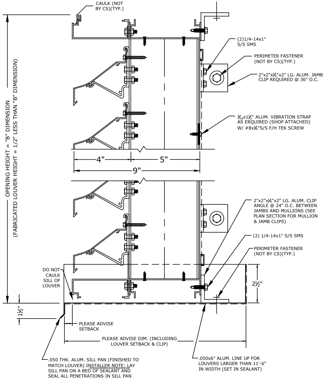
VERTICAL SECTION (SEE SHEET 1 FOR PLAN SECTION) (NTS)
