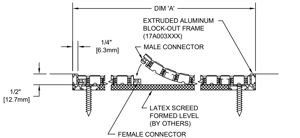
SECTION X-X
