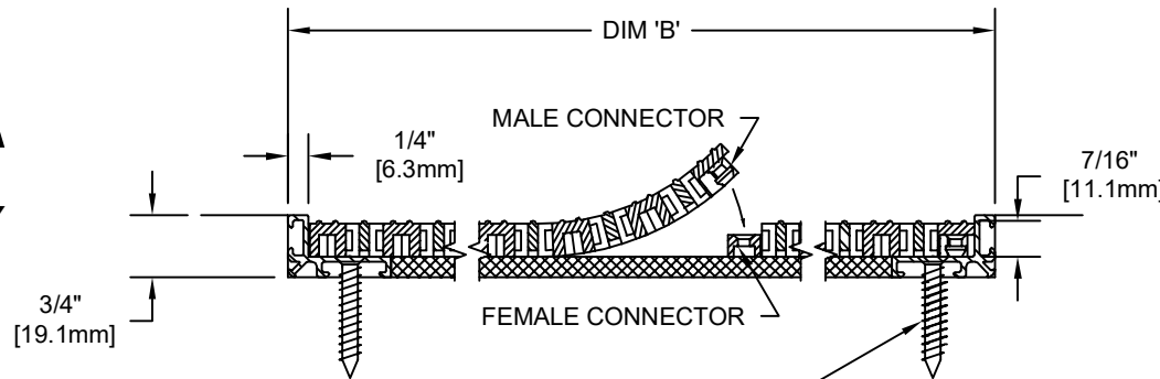
SECTION X-X
