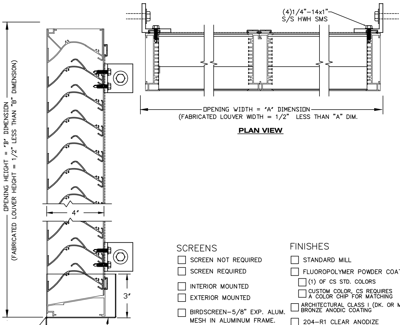
SECTION VIEW
