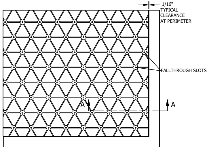
PLAN VIEW SCALE 1:5
