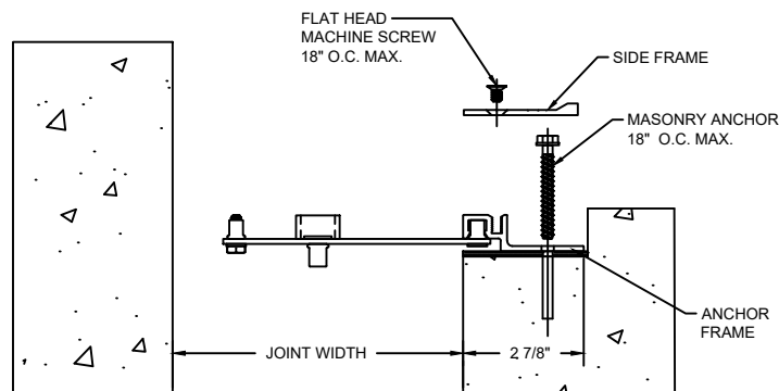
MODELS - SJPFW 700/800 WITH TURNBARS
