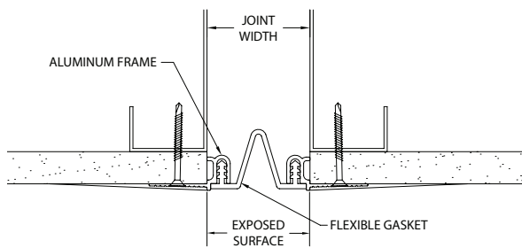
FWS-200
