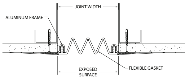
FWS-300/400
