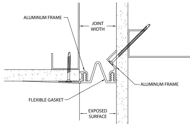
FWSC-200
