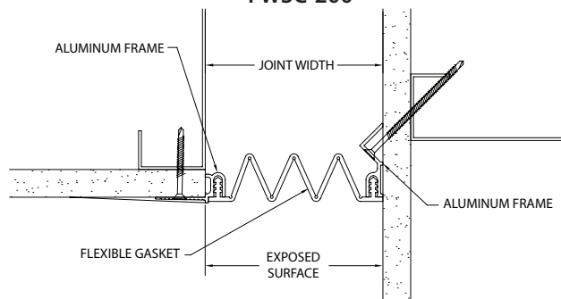
FWSC-300/400
