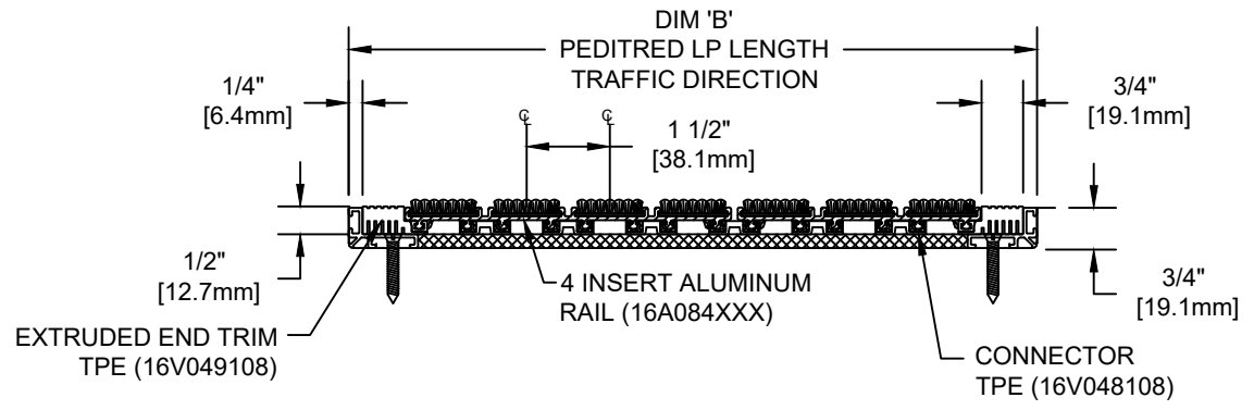
SECTION Y-Y
