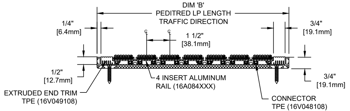
SECTION Y-Y
