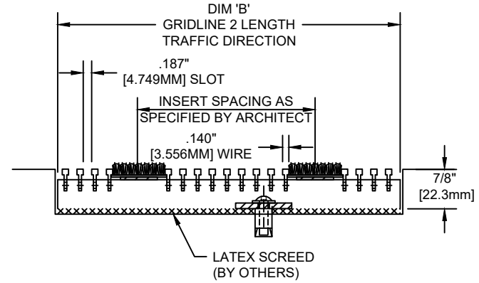
SECTION Y-Y
