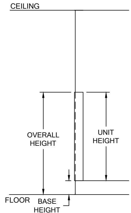
LG-200 CORNER GUARD AT PARTIAL HEIGHT ELEVATION
