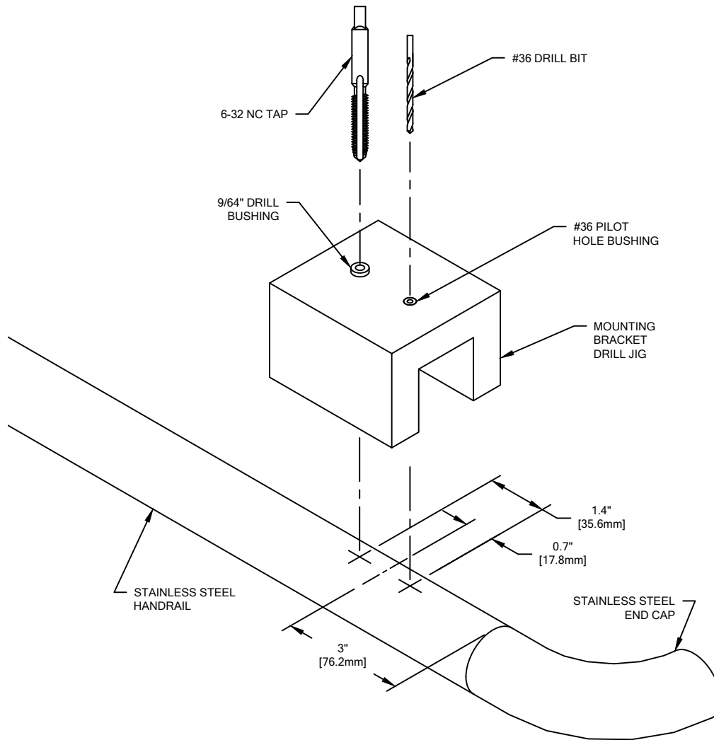
FIGURE 2. MOUNTING BRACKET DRILL JIG
