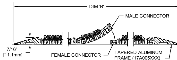
SECTION Y-Y
