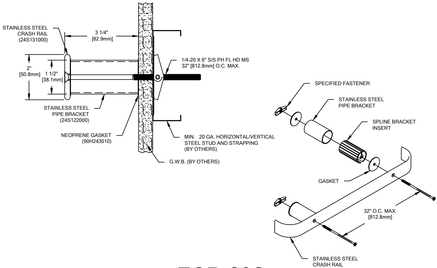
TYPICAL ASSEMBLY
