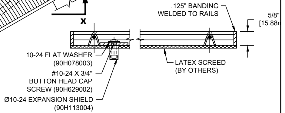
SECTION X-X NOT TO SCALE
