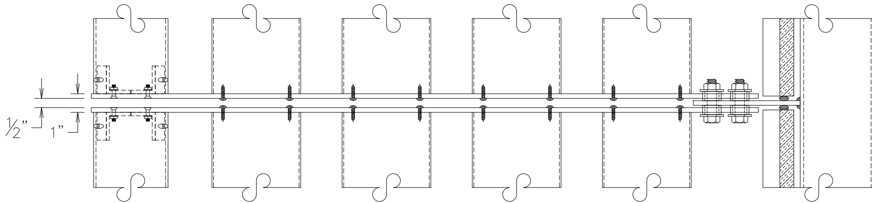
PLAN VIEW DETAIL OF CUSTOM CANTILEVER AIRFOIL SUNSHADE SYSTEM
