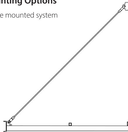
Mounting clips bolt to the face of the structure and tension rods
