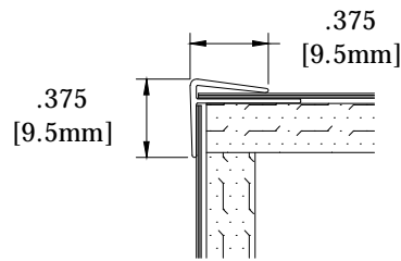
OUTSIDE CORNER (25N032XXX)
