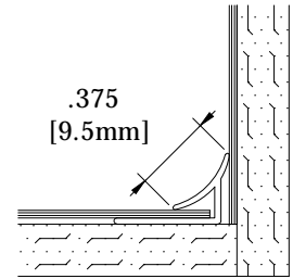
INSIDE CORNER (25N035XXX)
