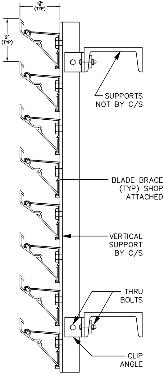
SECTION VIEW
