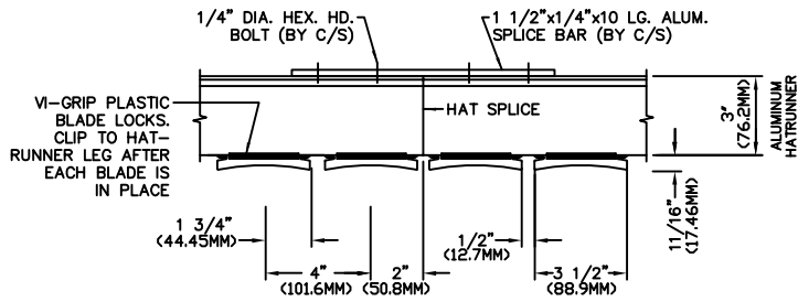
TYP SPLICE & BLADE SPACING DETAIL RF-20
