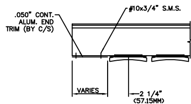
TYP. END DETAIL
