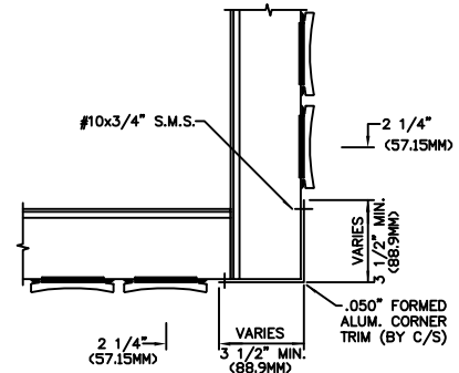
TYP. OUTSIDE CORNER DETAIL
