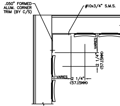
TYP. INSIDE CORNER DETAIL RF-20
