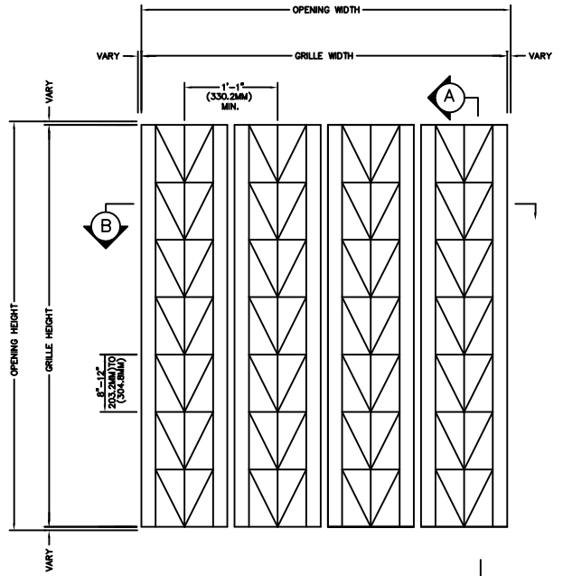
EXTERIOR ELEVATION
