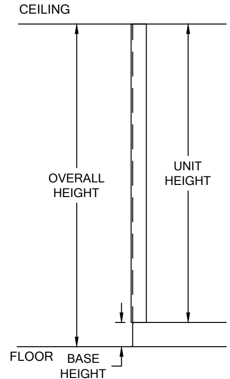
LG-150M CORNER GUARD AT FULL HEIGHT ELEVATION
