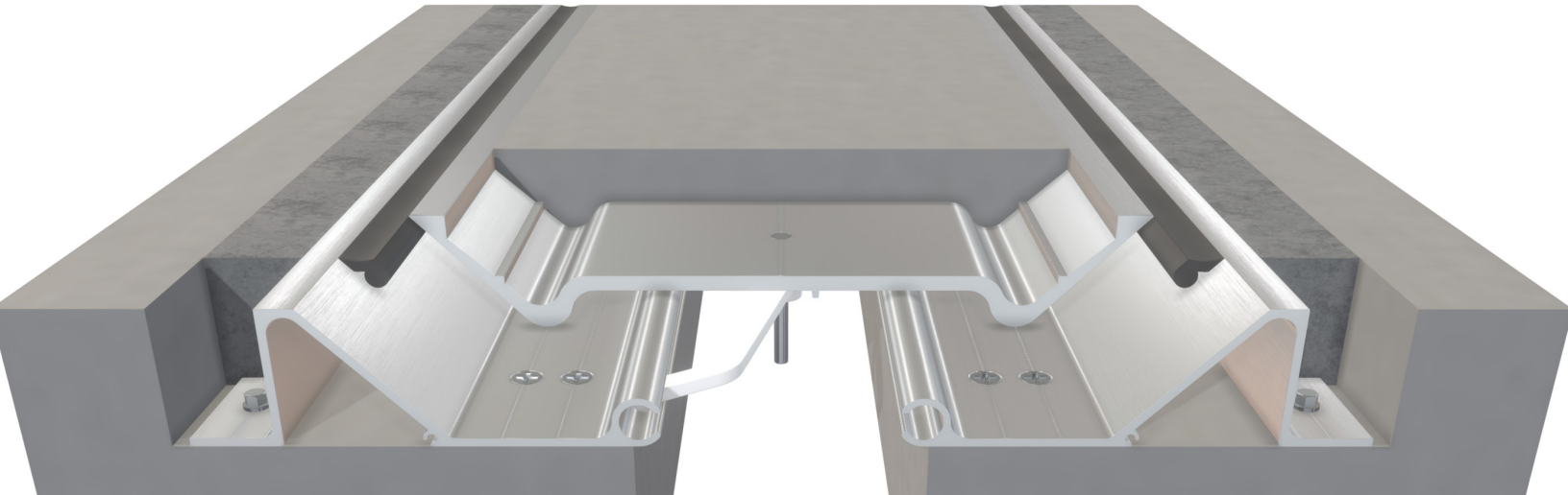
Model SSR-400
