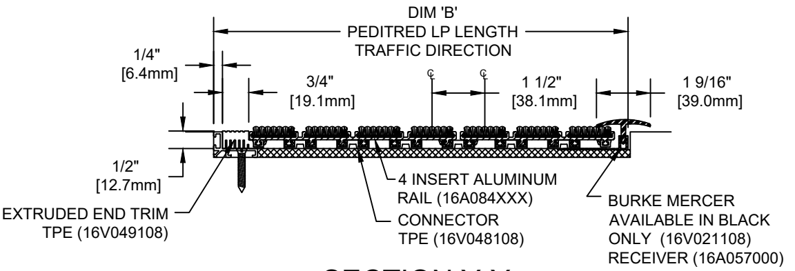
SECTION Y-Y
