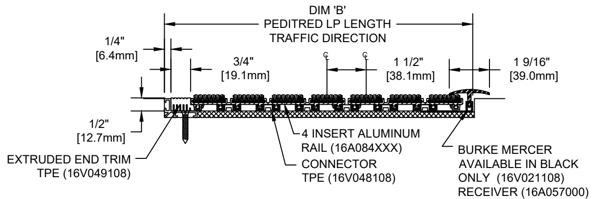
SECTION Y-Y
