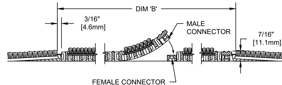
SECTION Y-Y
