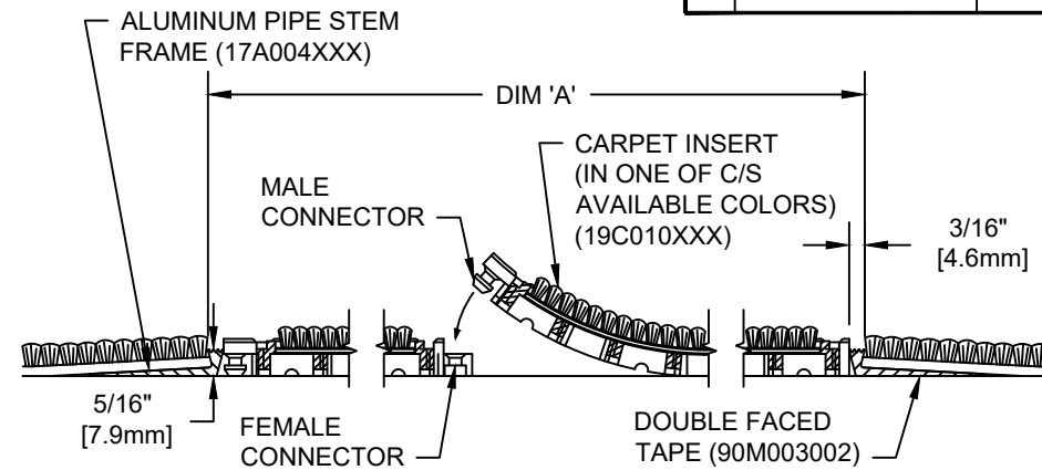
SECTION X-X
