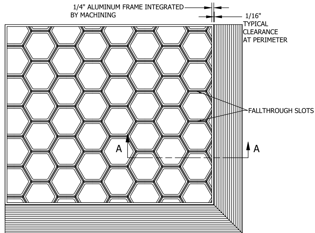
PLAN VIEW SCALE 1:5
