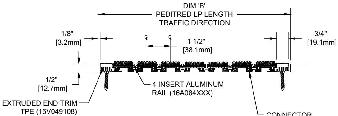
SECTION Y-Y
