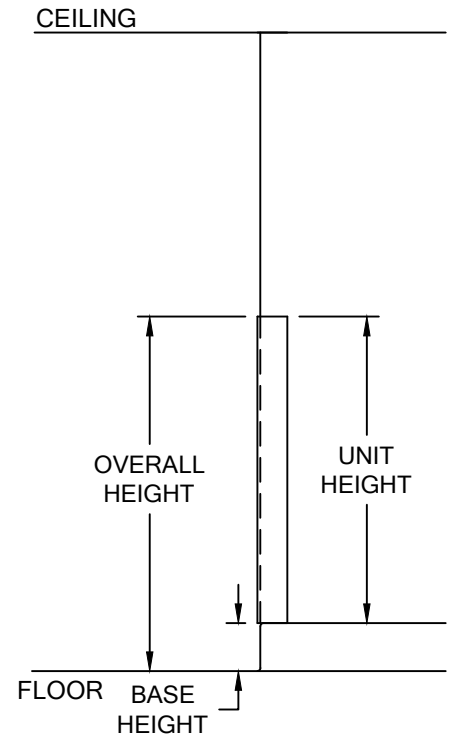
LG-150 CORNER GUARD AT PARTIAL HEIGHT ELEVATION
