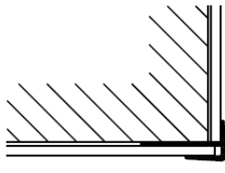
Standard Outside Corner Trim
