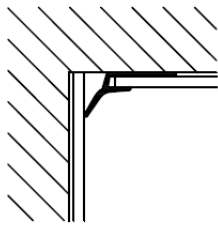
Inside Corner Trim
