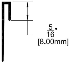
Wainscot Trim (25A023XXX)
