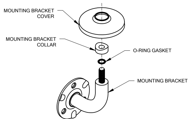
FIGURE 2. MOUNTING BRACKET ASSEMBLY
