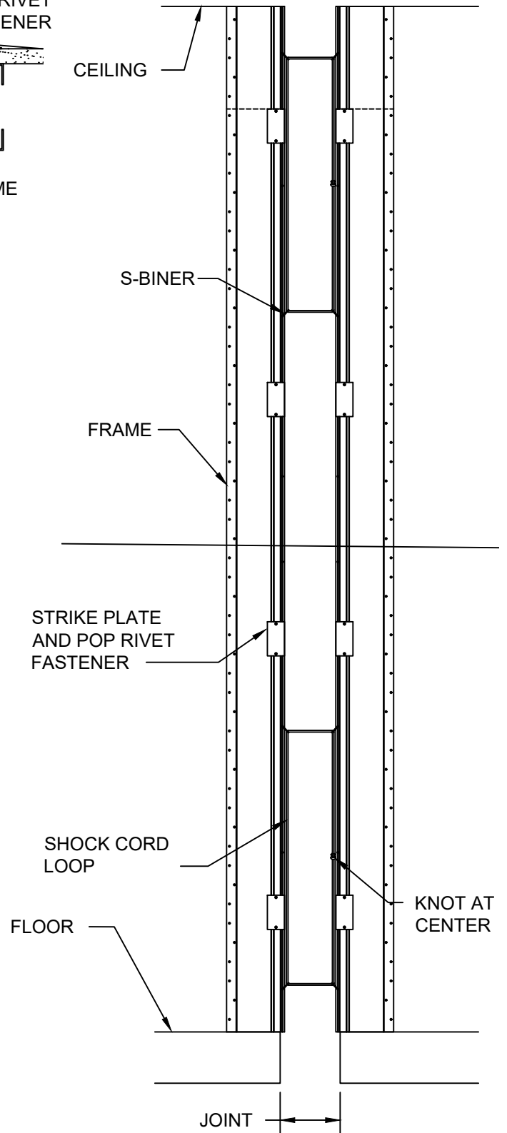
WALL ELEVATION
