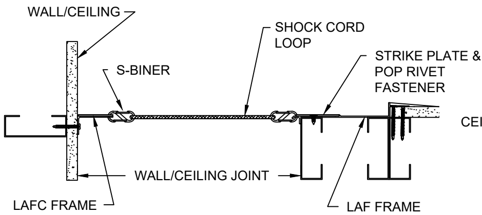
WALL/CEILING SECTION
