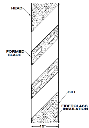
SECTION VIEW
