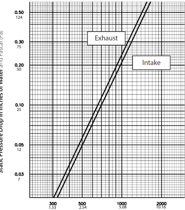
Free Air Velocity in Feet per minute and Metre per Second (m/s)
