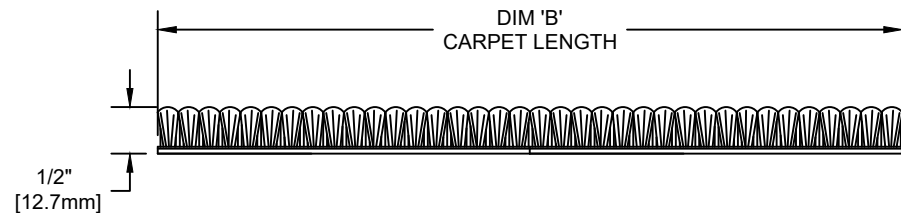
SECTION Y-Y
