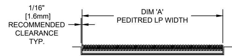
SECTION Y-Y
