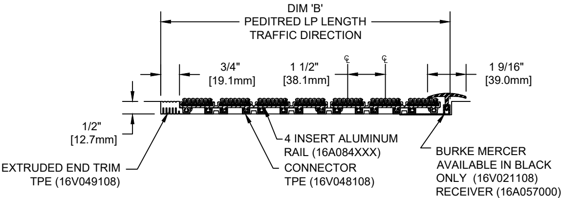
SECTION Y-Y
