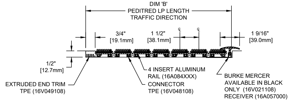
SECTION Y-Y
