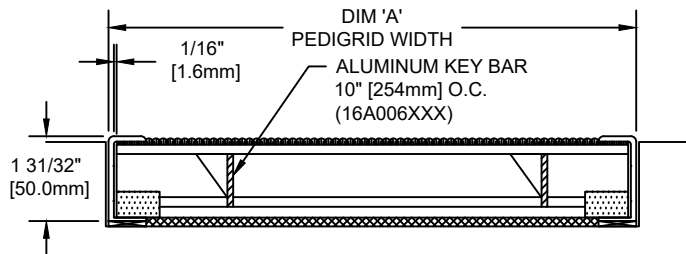
SECTION X-X
