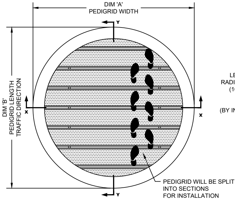
TYPICAL PLAN VIEW
