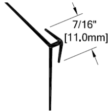
135° Outside Corner Trim (25A013001)
