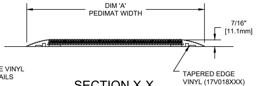
SECTION X-X
