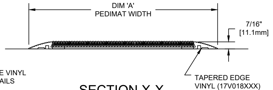
SECTION X-X
