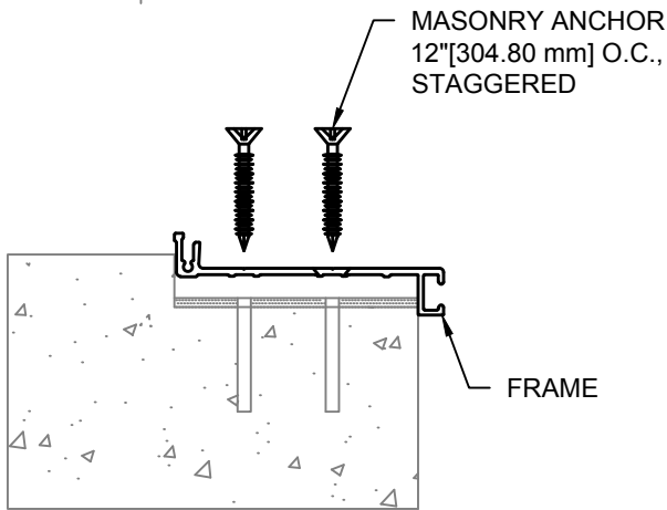
MODELS GTPW/GTRW
