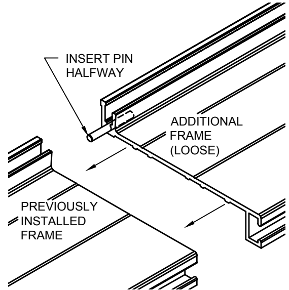
MODELS GTP/GTR
