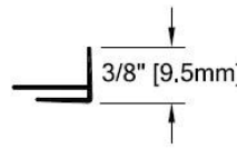
Outside Corner Trim (25N032xxxS, for .040/.060" sheet) (25N037xxxS, for .075" sheet)
