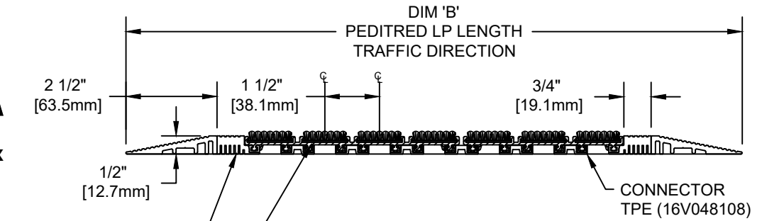
SECTION Y-Y
