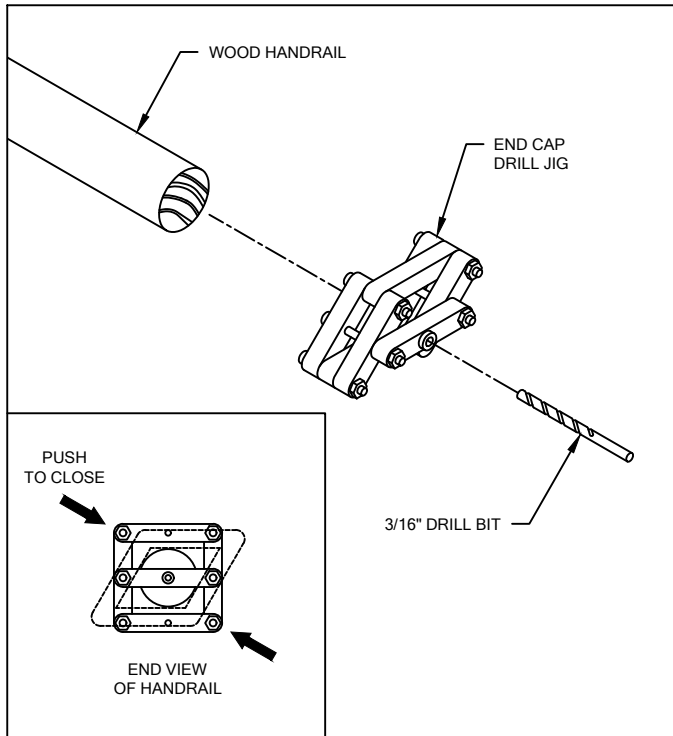
FIGURE 4. OPTIONAL STAINLESS STEEL SPLICE DRILL JIG
