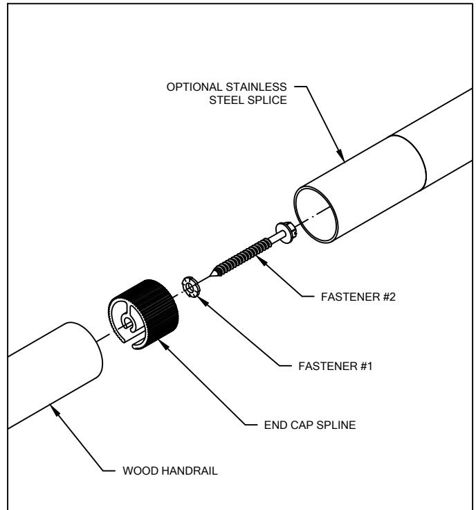
FIGURE 5. OPTIONAL STAINLESS STEEL SPLICE ASSEMBLY
