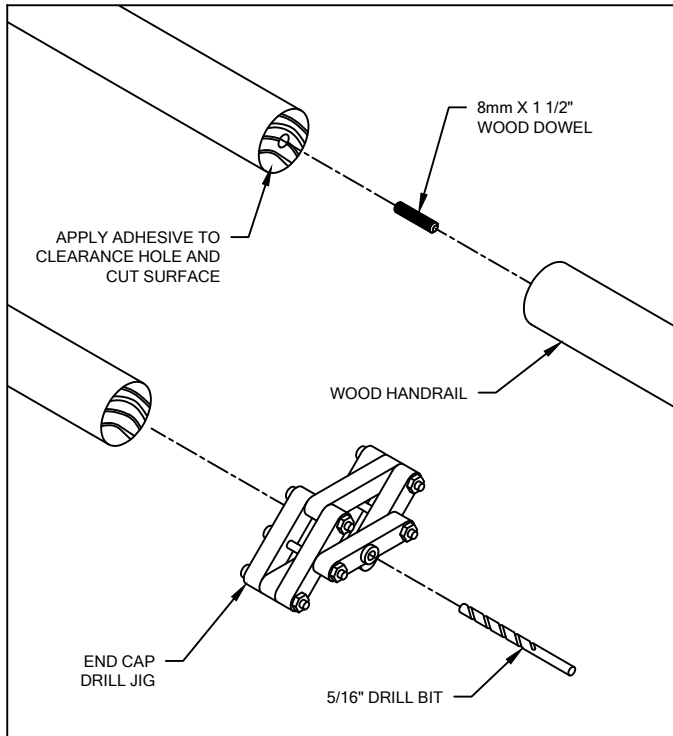
FIGURE 2. END CAP/CORNER DRILL JIG AND WOOD DOWEL SPLICE
