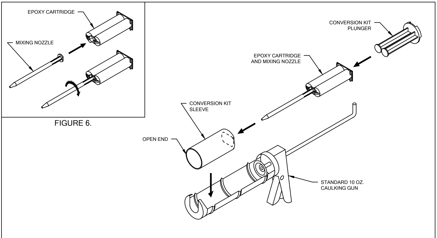
FIGURE 7. CAULKING GUN CONVERSION KIT
