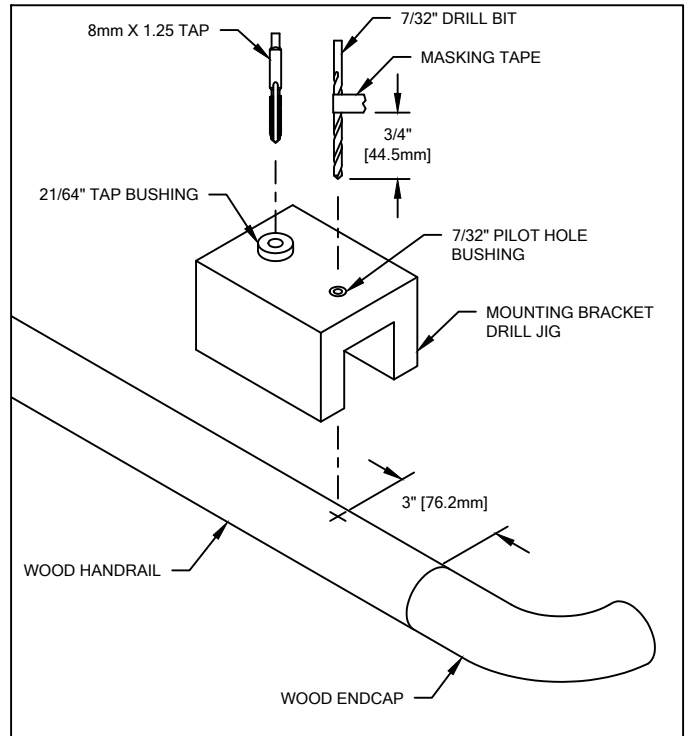
FIGURE 3. MOUNTING BRACKET DRILL JIG
