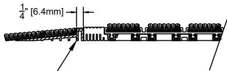
ALUMINUM PIPESTEM FRAME (16A048000)
