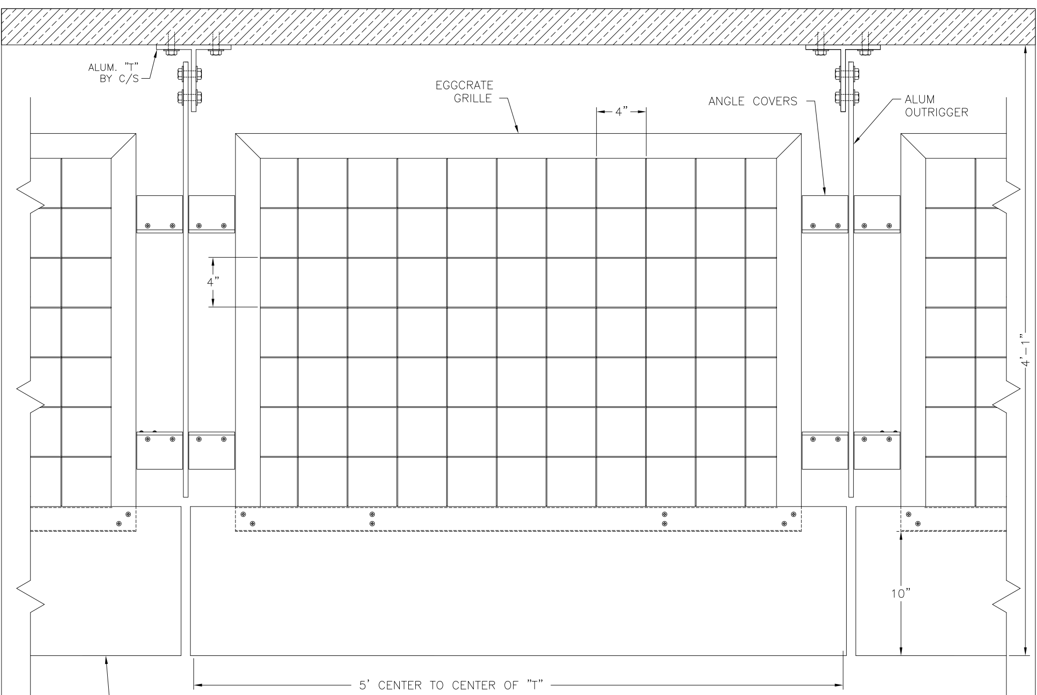
PLAN VIEW
