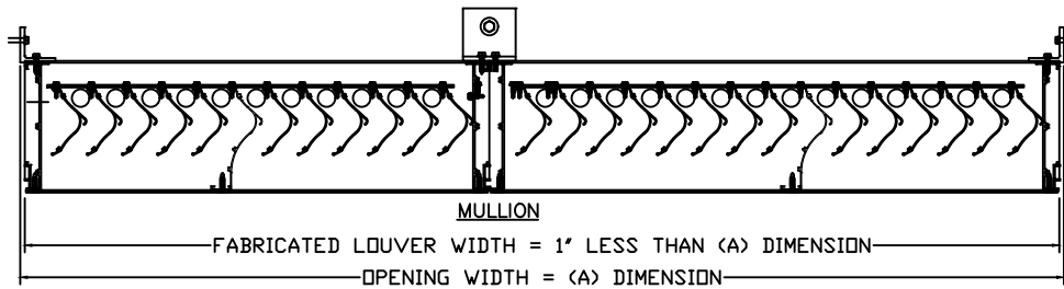
PLAN VIEW
