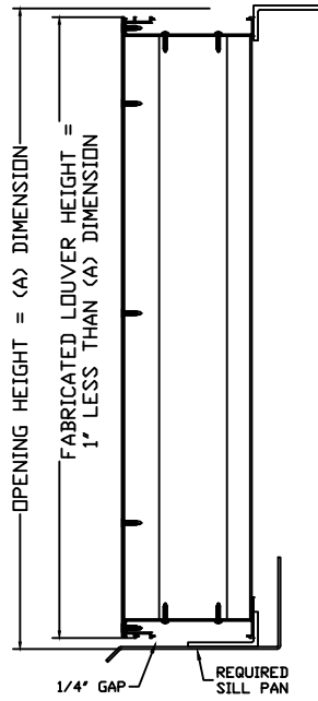
VERTICAL SECTION
