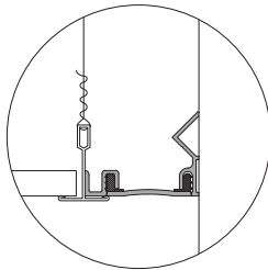
Ceiling to Wall Flat
