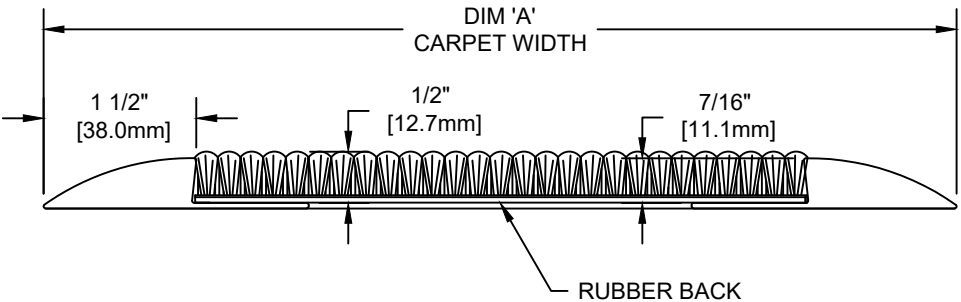
SECTION X-X
