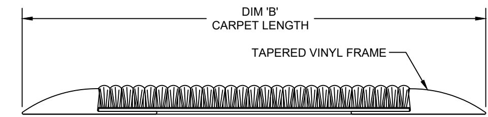
SECTION Y-Y
