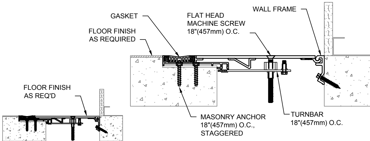
MODEL SGPW
