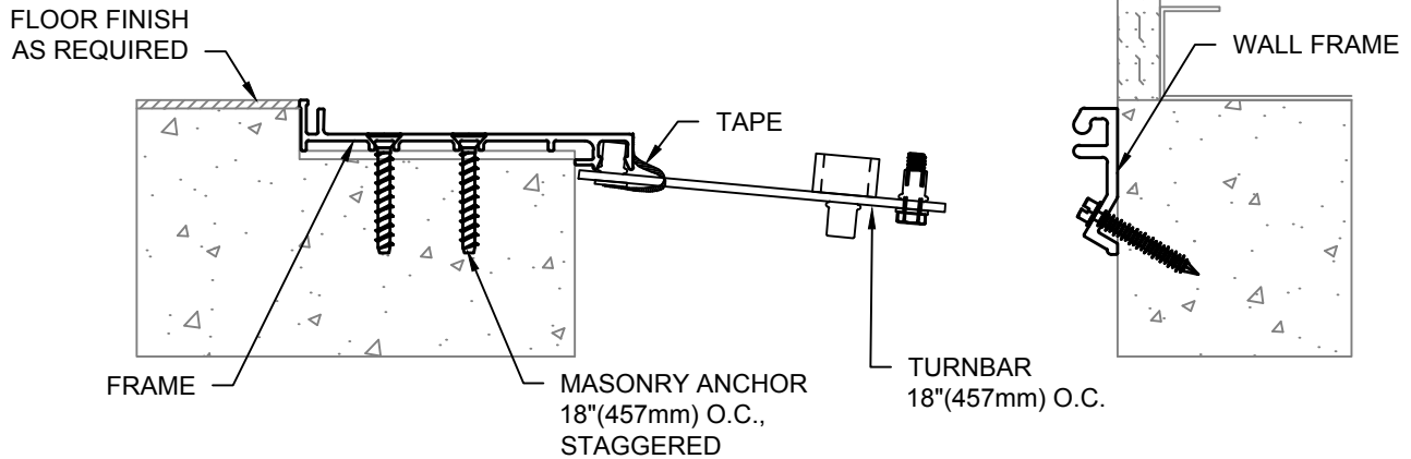
MODEL SGPW/SGRW
