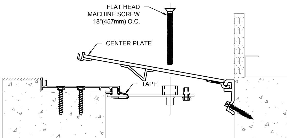
MODEL SGRW
