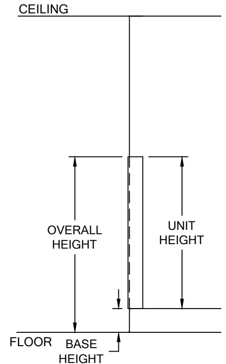
LG-150M CORNER GUARD AT PARTIAL HEIGHT ELEVATION
