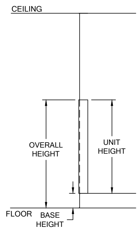
LG-300 CORNER GUARD AT PARTIAL HEIGHT ELEVATION
