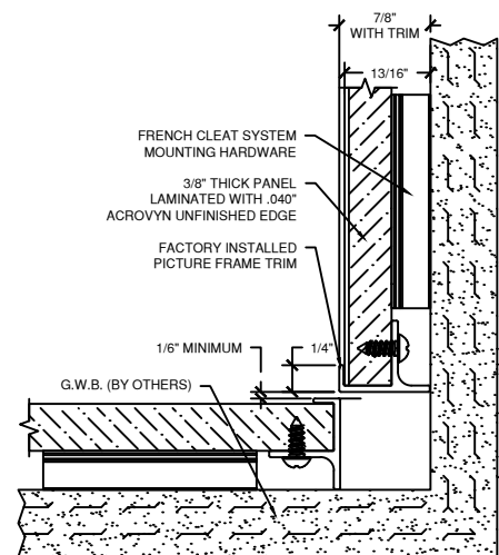
(G) BUTTED INSIDE CORNER OPTION
