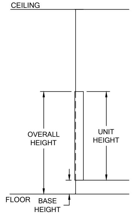
LG-200M CORNER GUARD AT PARTIAL HEIGHT ELEVATION
